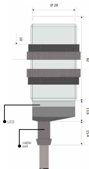
C30*/**-*A (cable exit)
