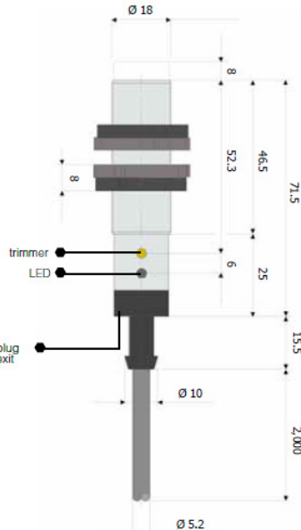
C30*/**-*A (cable exit)
