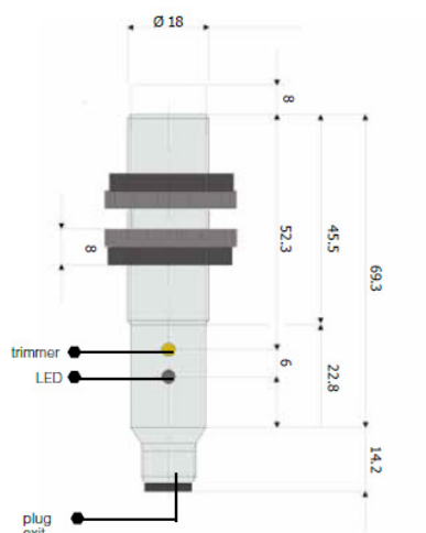
C18*/**-*E (plug exit)
