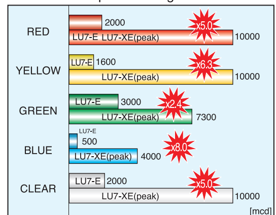
Comparative Brightness
