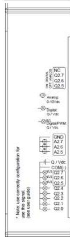
Configuration Switch* (see section 8 to select the correct configuration for outputs).
