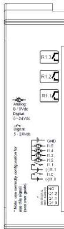
RELAY Outputs
