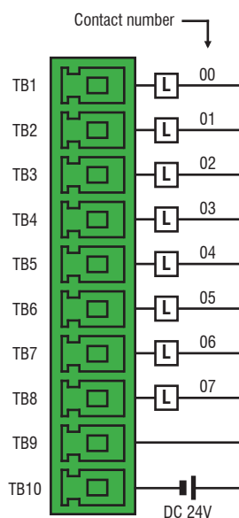
8 Point Sink Output XBE-TN08A
