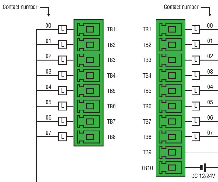
16 Point Sink Output XBE-TN16A
